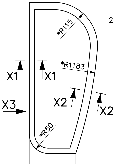
ITEM-15 (1:5)
