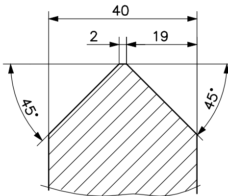
SECTION-X1X1 (1:1)
