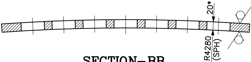
SECTION-BB (1:5)
