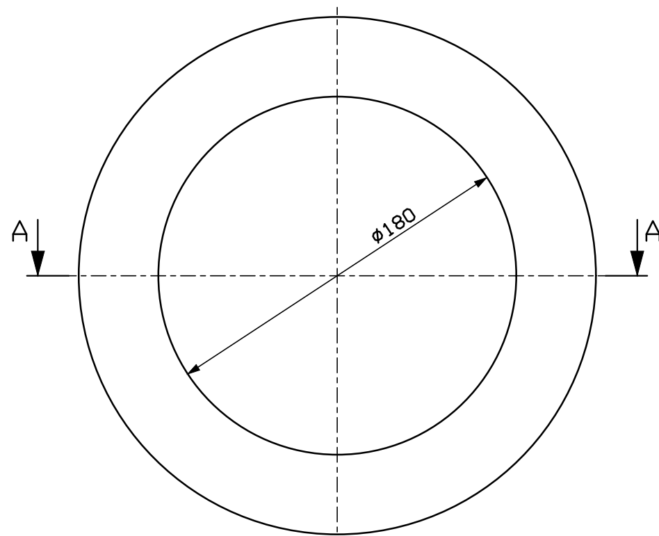
SLEEVE (1: 2.5)
