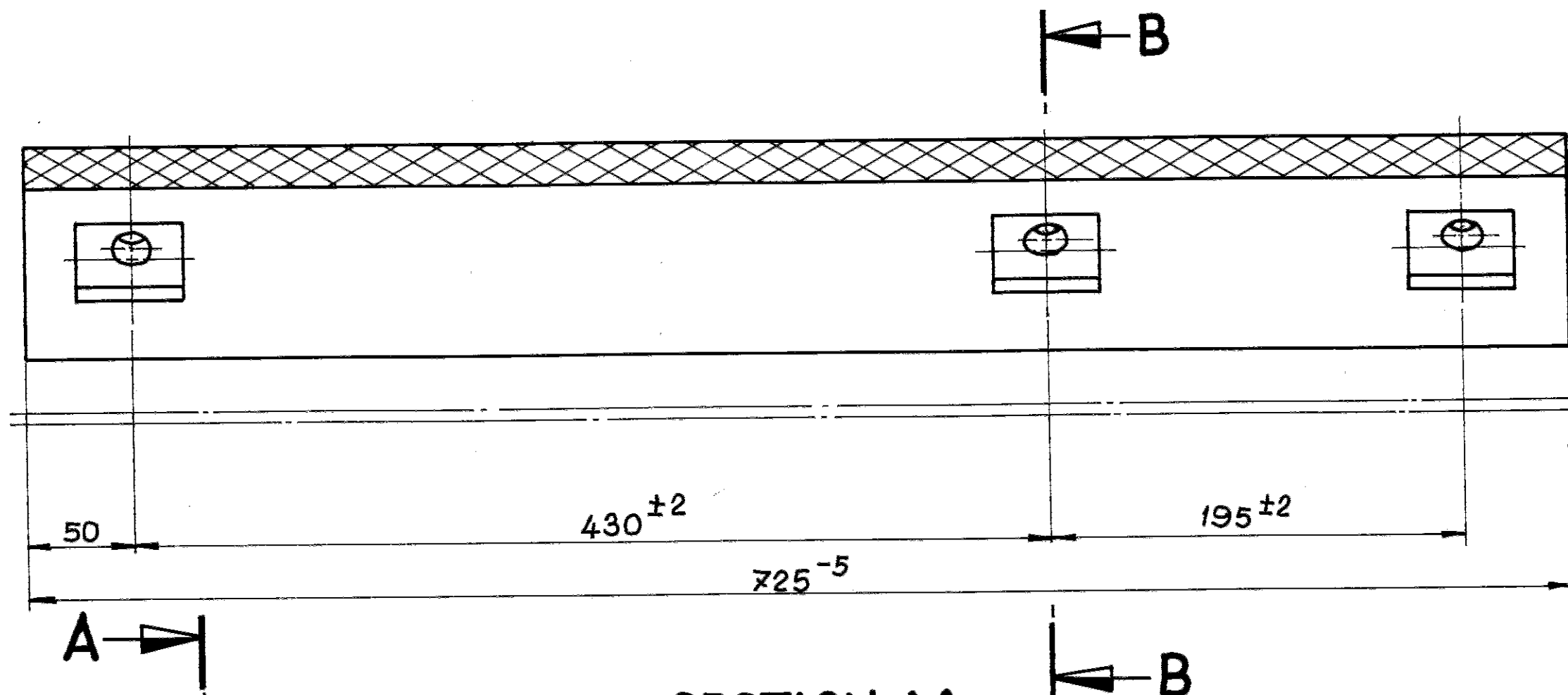
SECTION-AA
