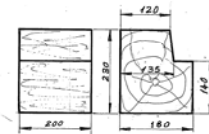
DETAIL II (ITEM NO. 7)
