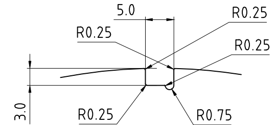
Detail B (2:1)
