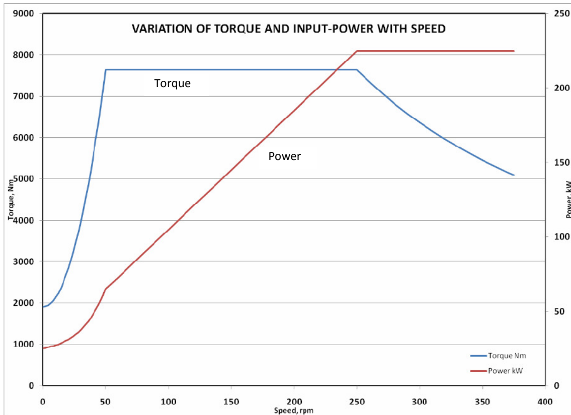
Fig.1: Torque Speed characteristics of variable speed 200 kW Synchronous Motor (UUT)
