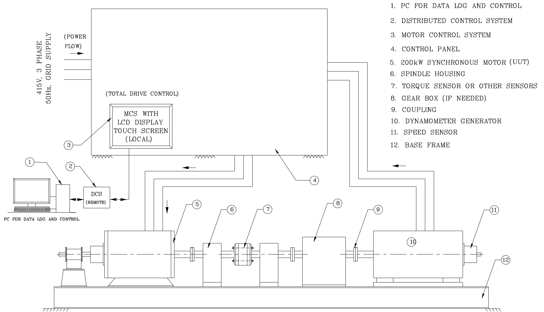
SCHEMATIC DIAGRAM OF 200kW SYNCHRONOUS MOTOR ENDURANCE TEST SET-UP
