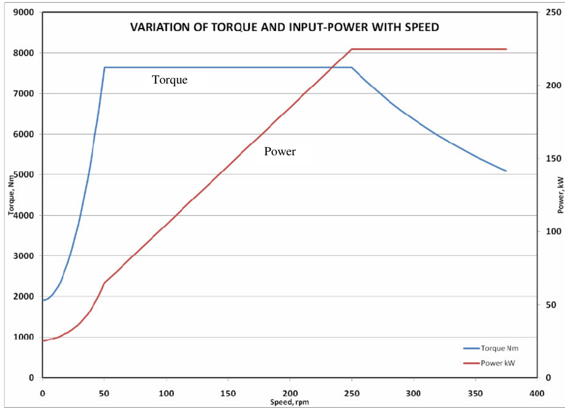
Figure1: Torque Speed characteristics of variable speed Synchronous motor
