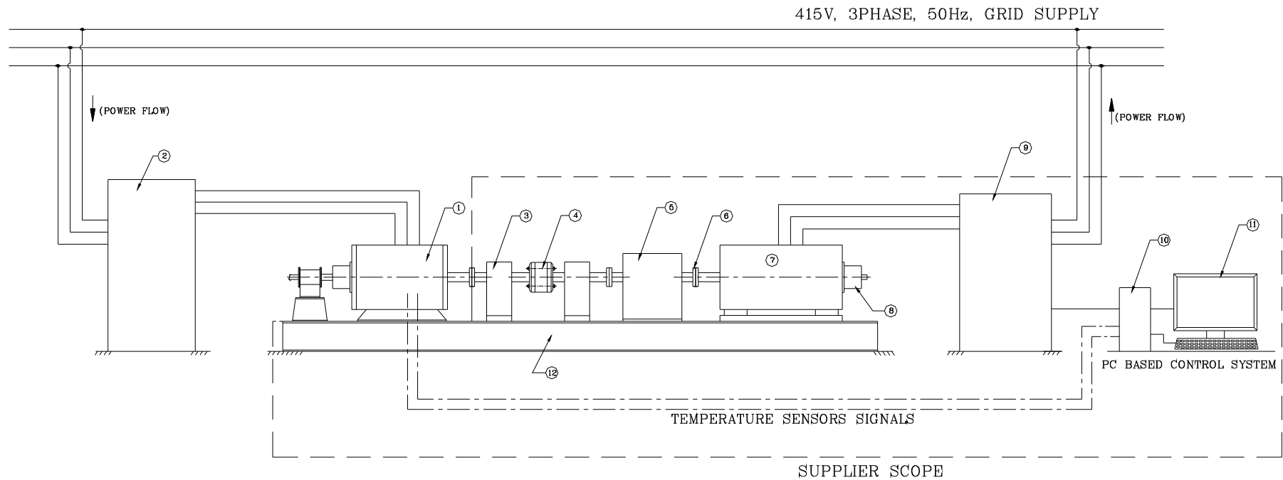
SCHEMATIC DIAGRAM OF 200kW SYNCHRONOUS MOTOR ENDURANCE TEST SET-UP
