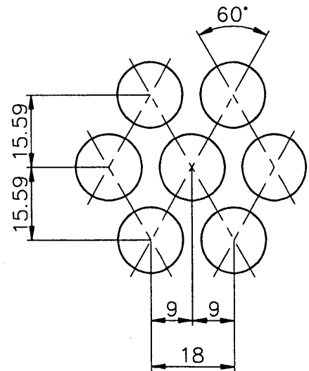
PITCH PATTERN
