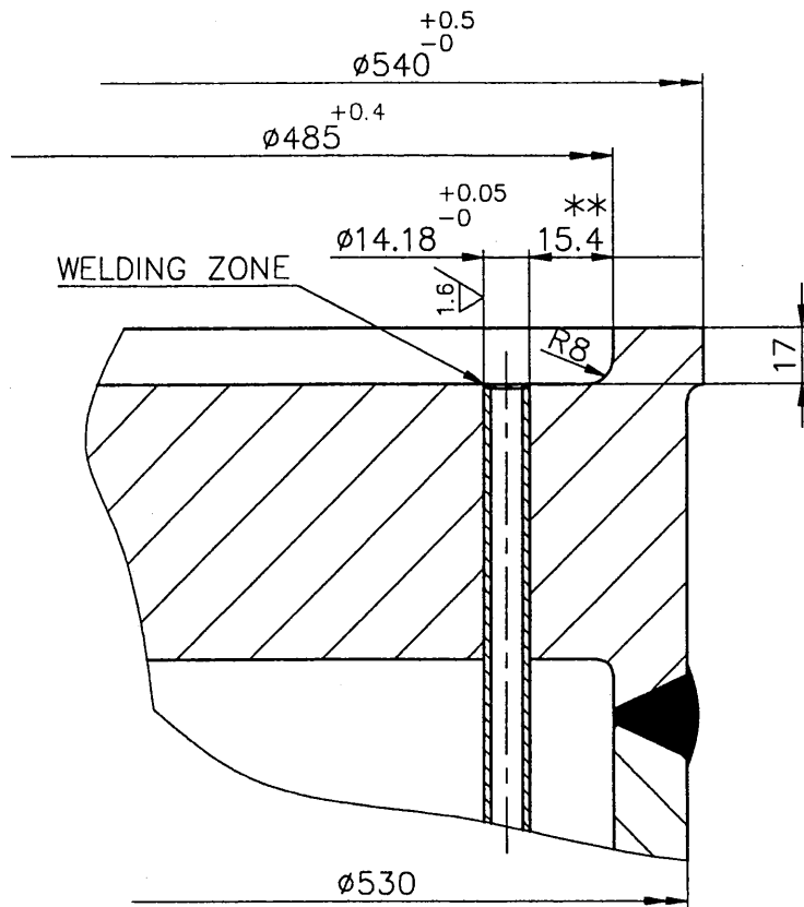
EP DETAIL
