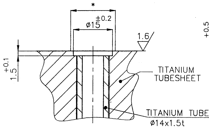
EP DETAIL
