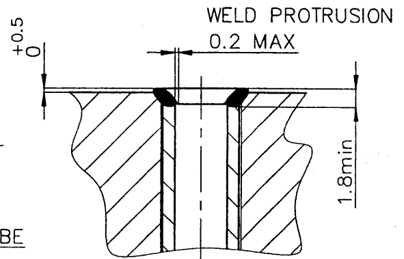
WELD DETAIL
