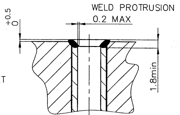
WELD DETAIL
