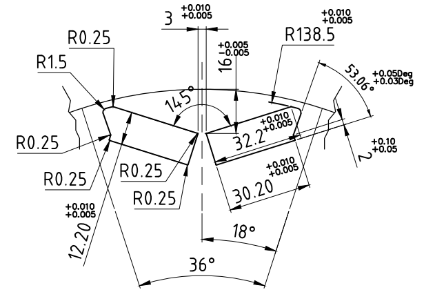
Detail A (10 Sets)
