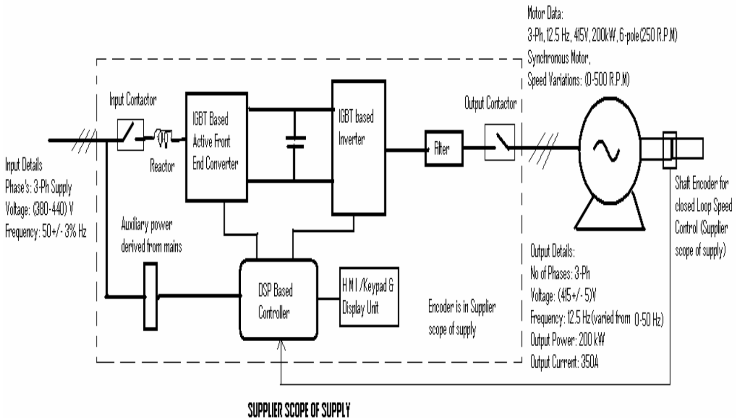
Fig 1: Single Line diagram of the VFD System with the input and output details.
