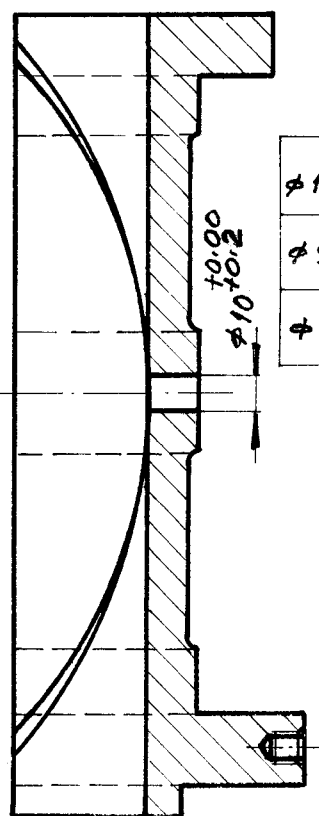
DETAIL P-P
