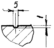
DETAIL D-D
