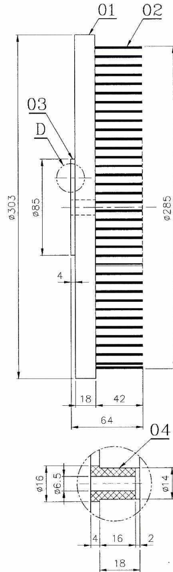
DETAIL- 'D'
