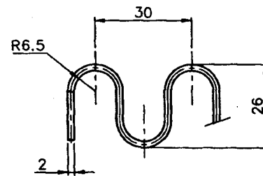
DETAIL-X
