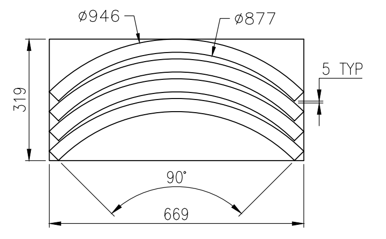
ITEM NO:2 CUTTING PLAN
