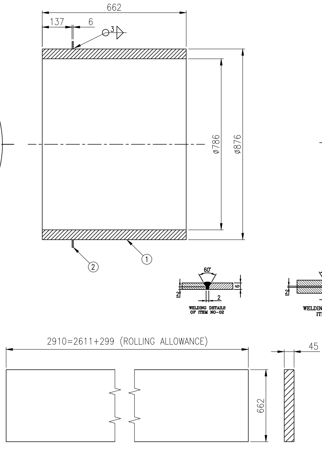
DEVELOPED LENGTH OF ITEM-01 SCALE 1:2
