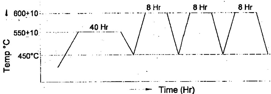
Fig 1: Simulated Heat Treatment
