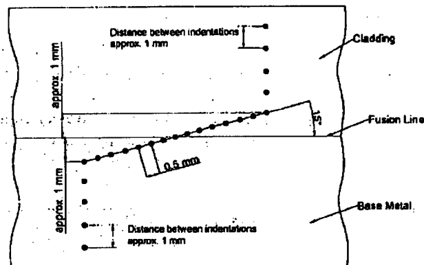
Fig 3: Hardness test
