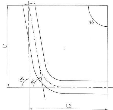
\theta_3 = \theta_2 = REQUIRED ANGLE OF BEND FIGURE –2
