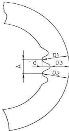
D – NOMINAL OD OF PIPE FIGURE –1
