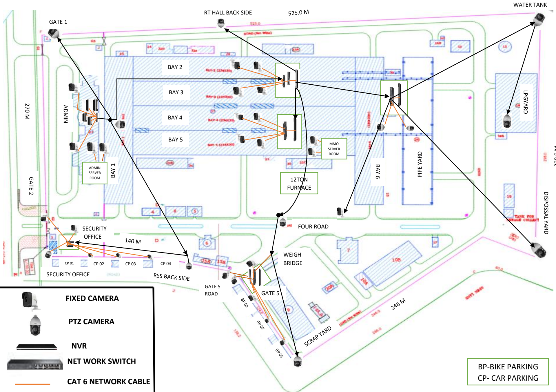
PPPU CCTV LAYOUT
