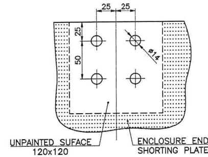
DETAIL-A (FOR IT-003 ONLY)
