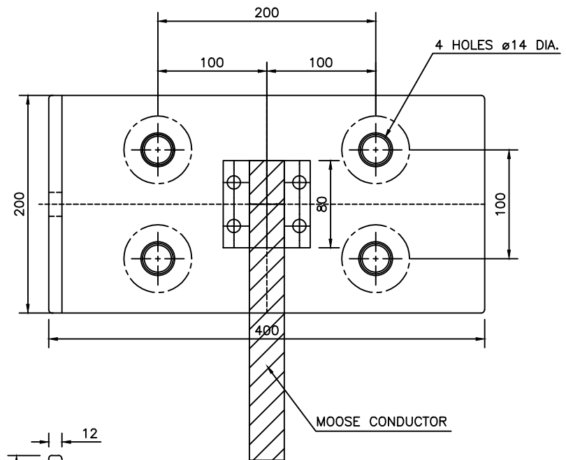
TOP VIEW WITH INSULATOR BASE
