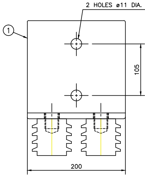
SIDE VIEW WITH INSULATOR BASE
