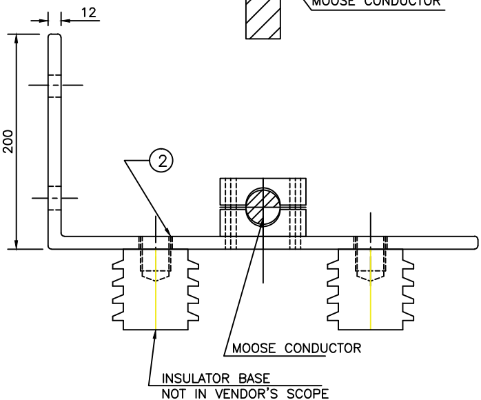
FRONT VIEW WITH INSULATOR BASE
