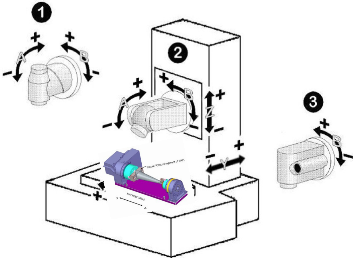
FIG 3 MACHINE AXES
