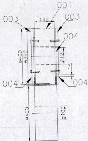
ROLLER ARRANGEMENT
