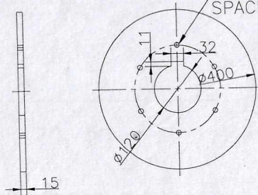
GUIDE PLATE 15TK QTY. 02 (IT.003)
