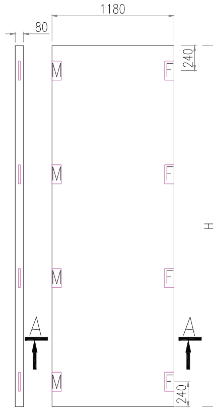
FLOOR PANEL
