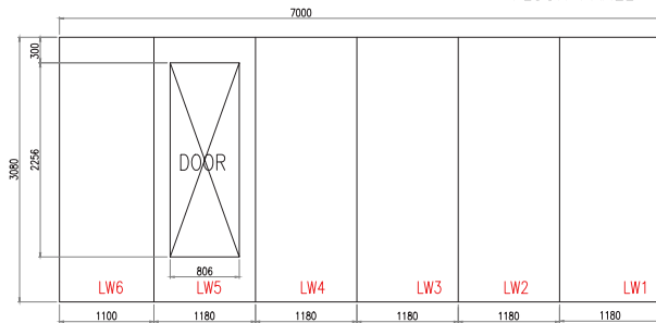
LEFT SIDE WALL
