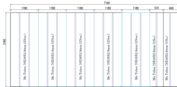
FLOOR PANEL
