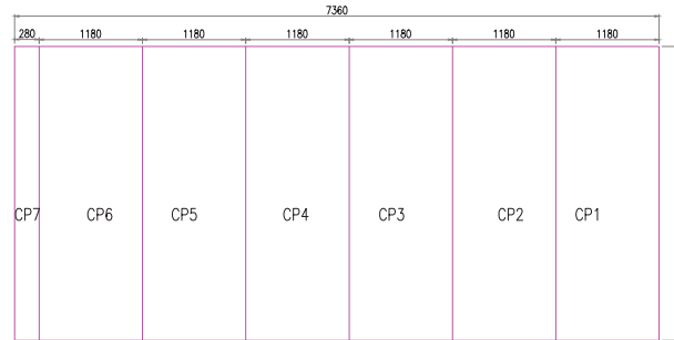
CEILING PANEL LAYOUT ROOF OVER HANG 100mm ALL SIDE
