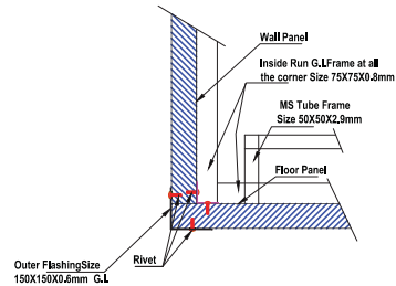
Tpy. :- Wall & Floor Panel Joint
