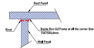
Tpy. :~ Wall & Roof Panel Joint DETAIL-D
