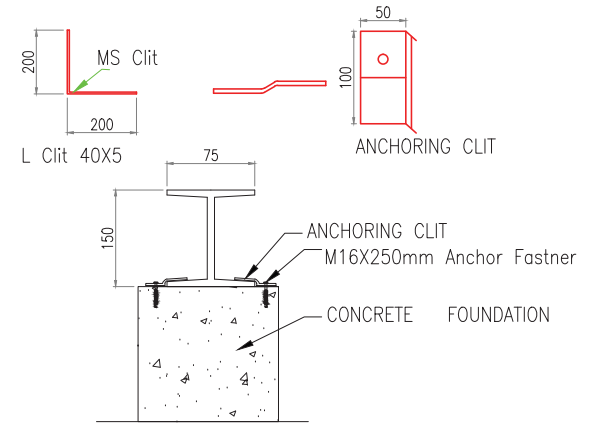
Base Fixing Arrangement
