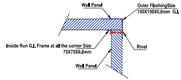
Typ. :~ Wall & Wall Panel Joint Corner Joint
