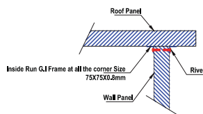
Tpy. :- Wall & Roof Panel Joint DETAIL-E
