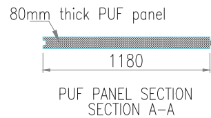
FLOOR PANEL
