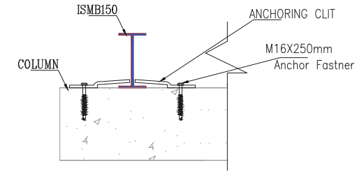
Base Fixing Arrangement
