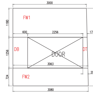
FRONT SIDE WALL
