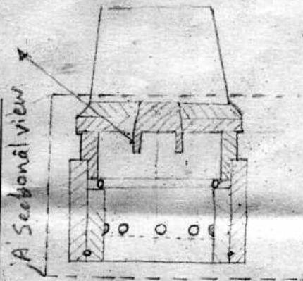
QUICK RELEASE COUPLING
