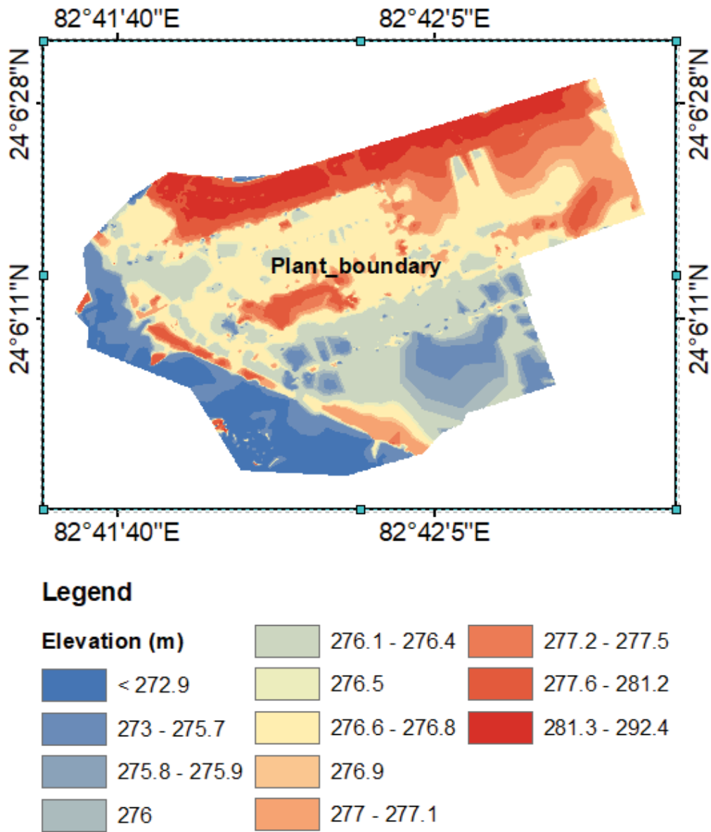
Figure 3.9 DEM map of the plant boundary
