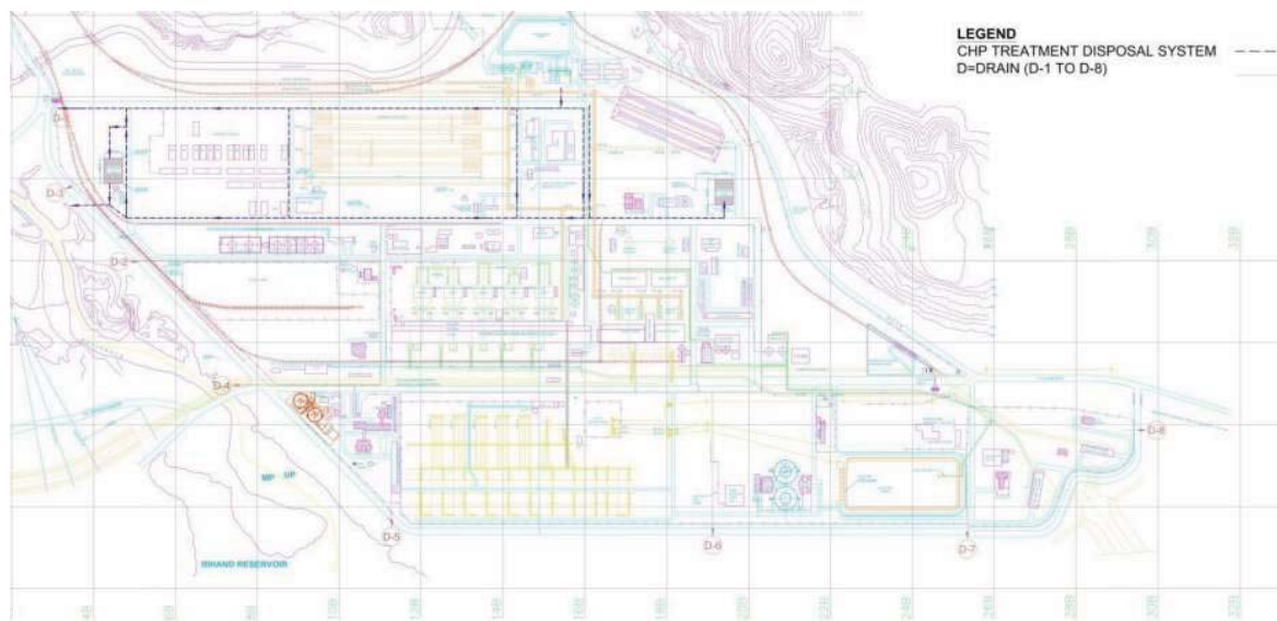
Figure 6.2 Existing drains and eight outfalls (D1 to D8)
