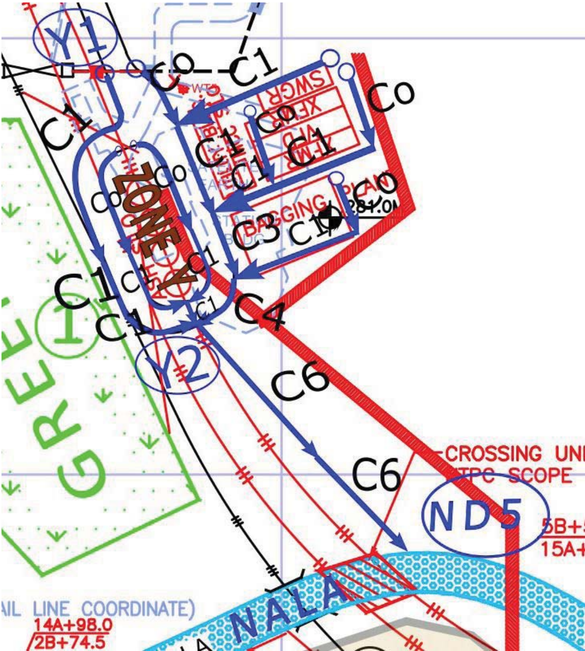
Figure 6.9 Layout of drains in Y zone
