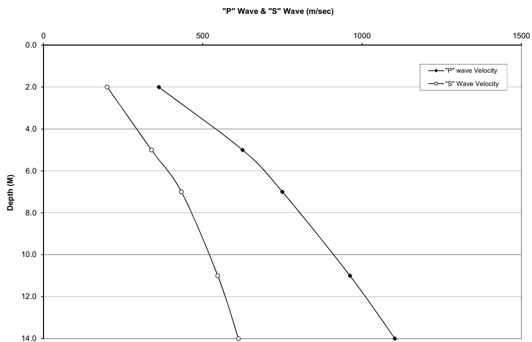
Variation of "P" &amp; "S" wave Velocity with Depth
