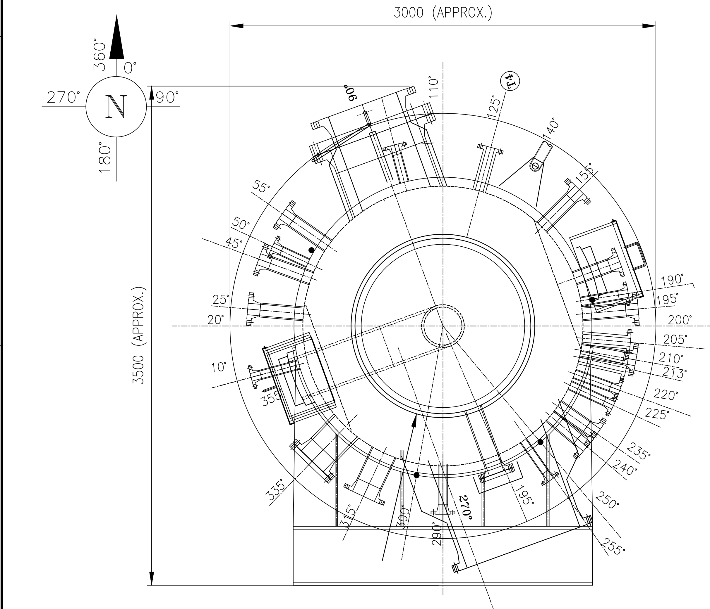
ORIENTAION OF SADDLE (VIEW FROM TOP)
