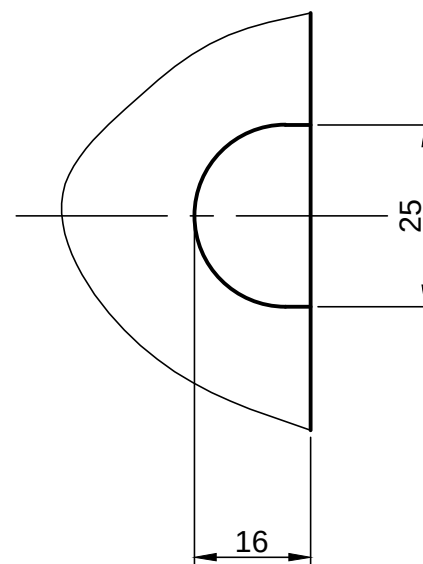
VIEW-Y
