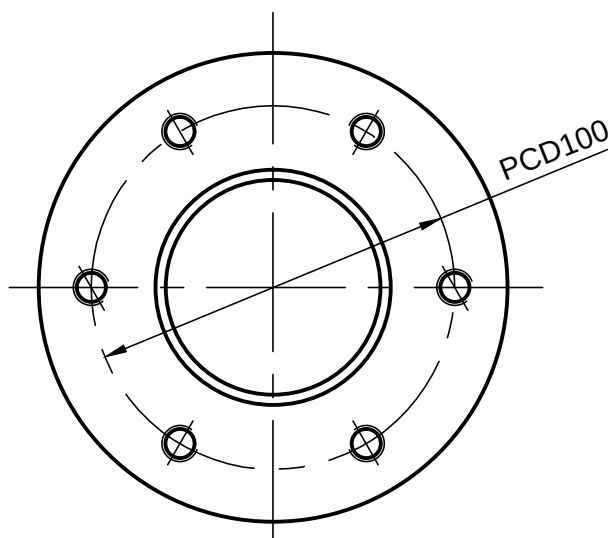
VIEW-X
