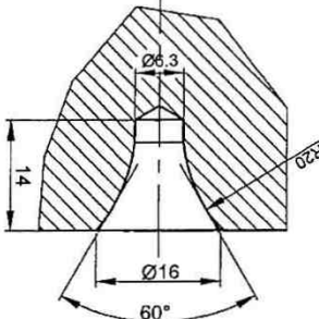
CENTRE DETAIL-C (SCALE 2:1)
