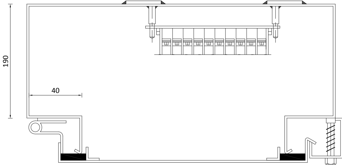
SECTION-XX
