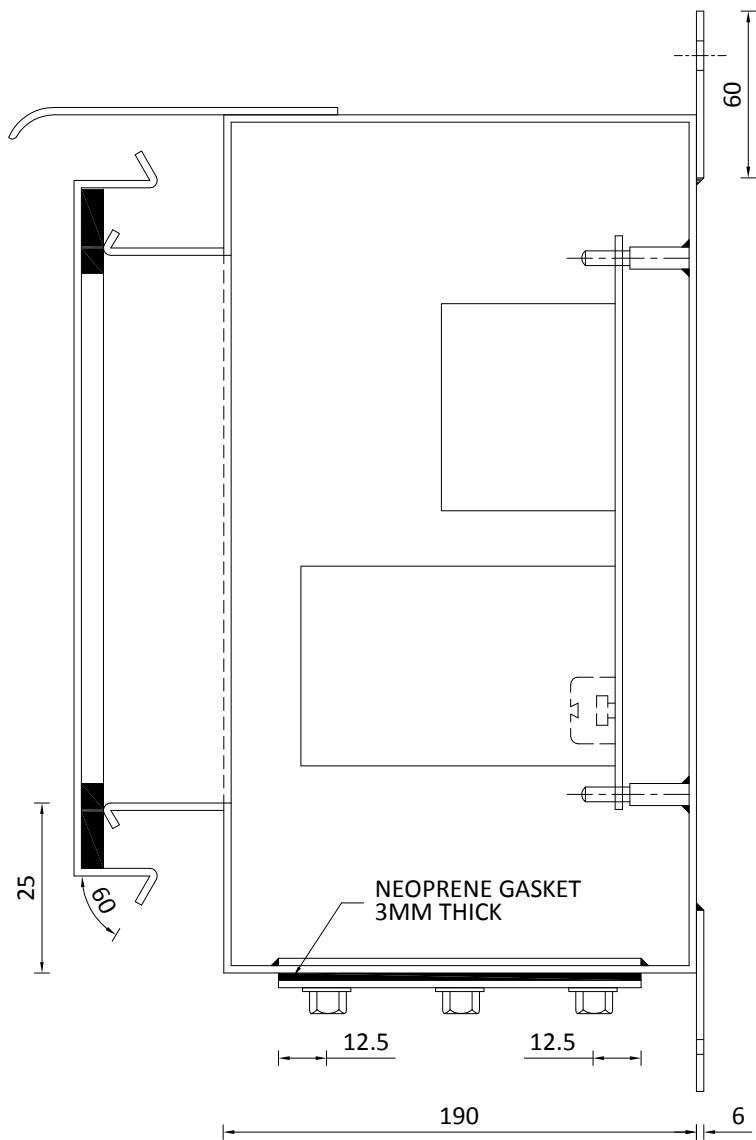
SECTION-YY
