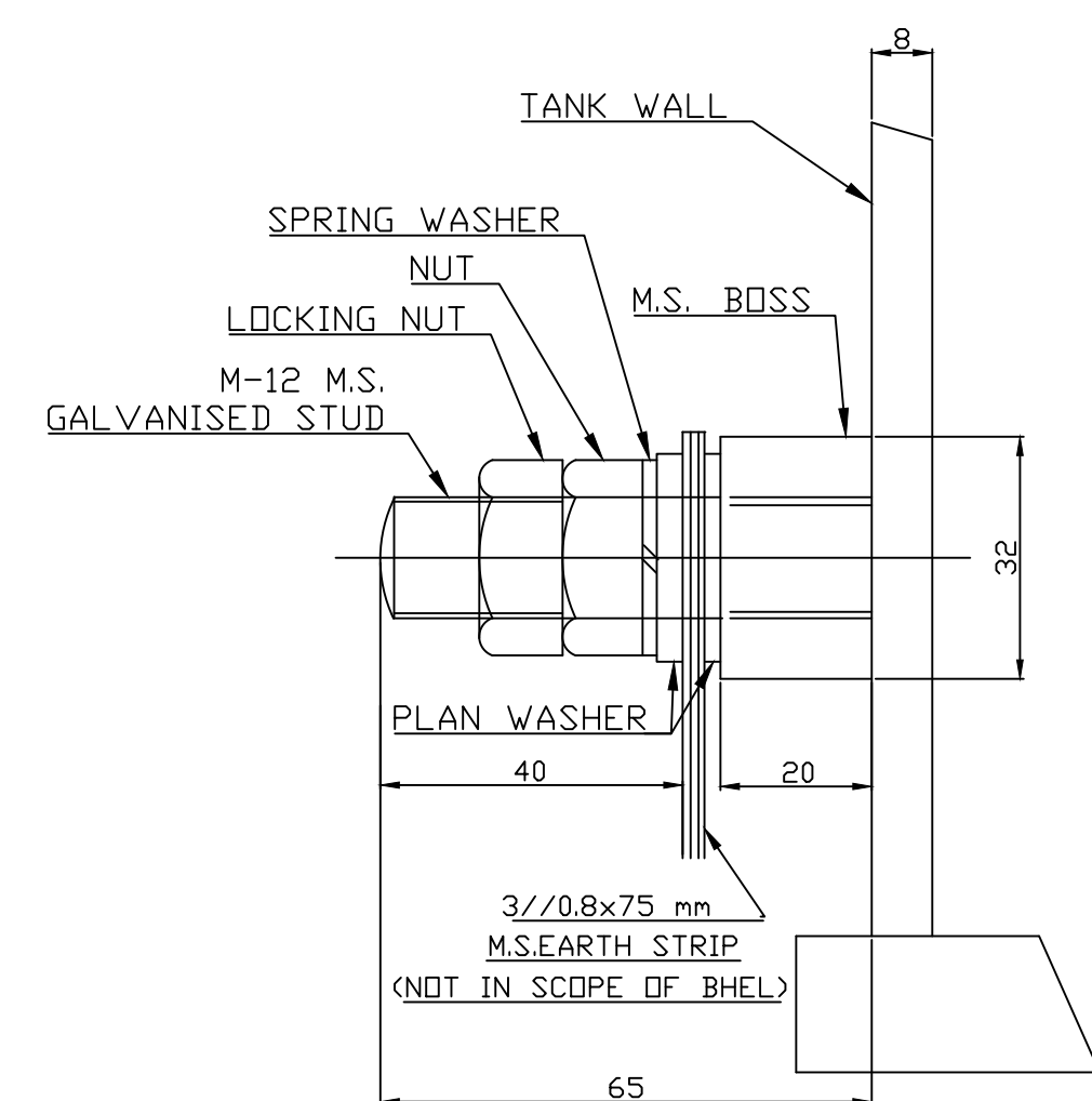
EQUIPMENT EARTHING DETAIL DETAIL-A
