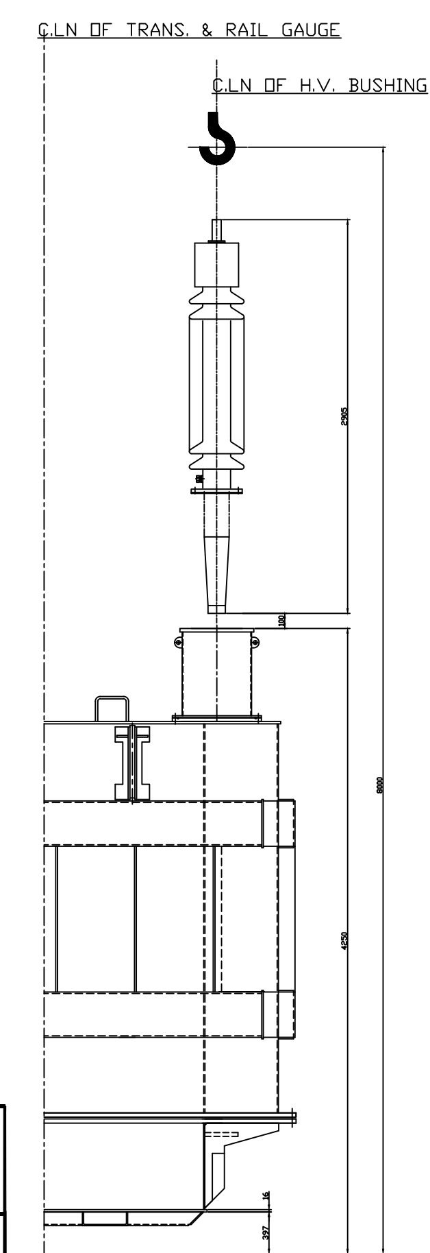
UN TANKING DETAIL OF H.V. BUSHING
