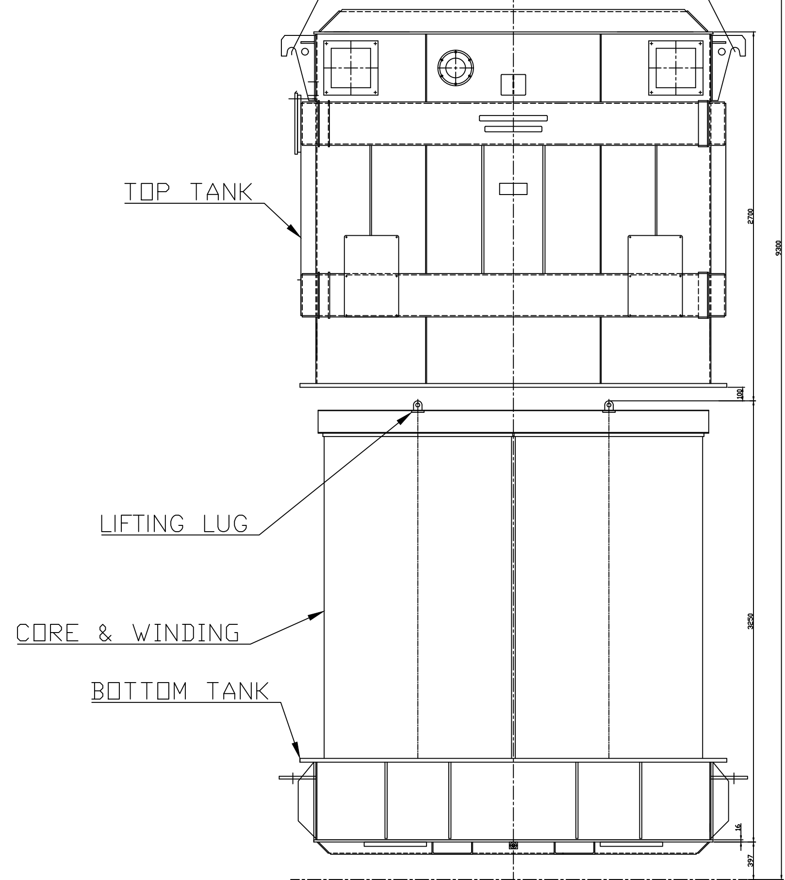
UN TANKING DETAIL OF TRANSF.
