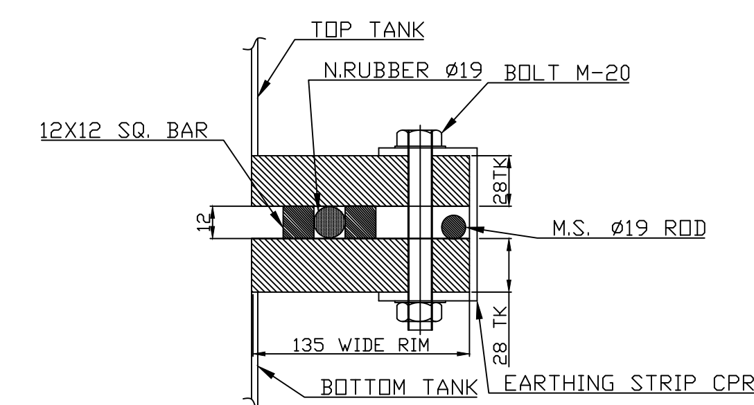
DETAIL-C TOP & BOTTOM TANK RIM ARRG
