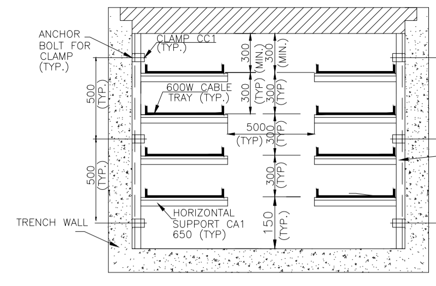
TRENCH DETAIL 1800WX1350D TR A-A
