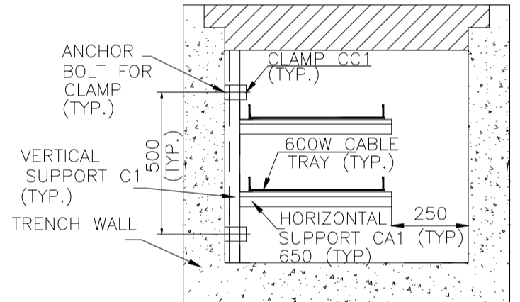
TRENCH DETAIL 900WX750D TR E-E
