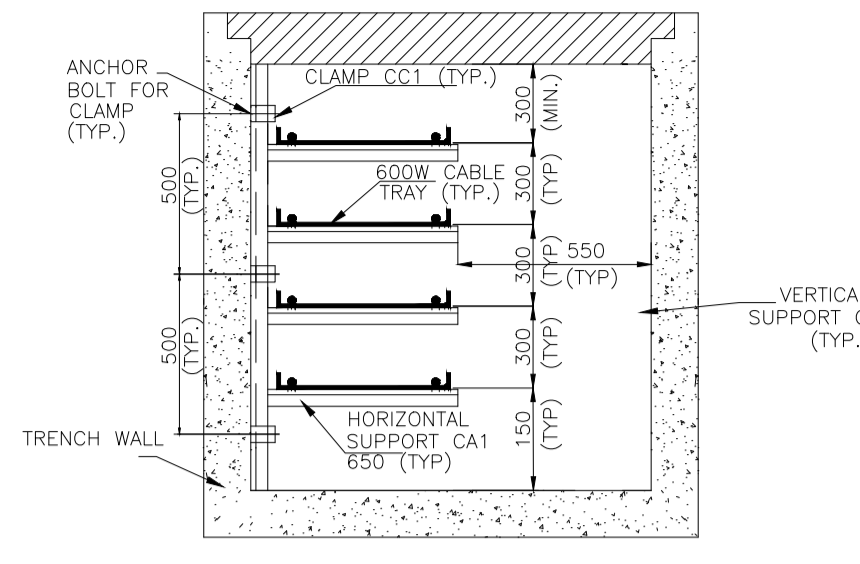
TRENCH DETAIL 1200WX1350D
