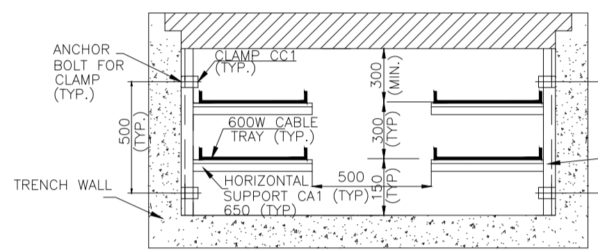
TRENCH DETAIL 1800WX750D TR B-B
