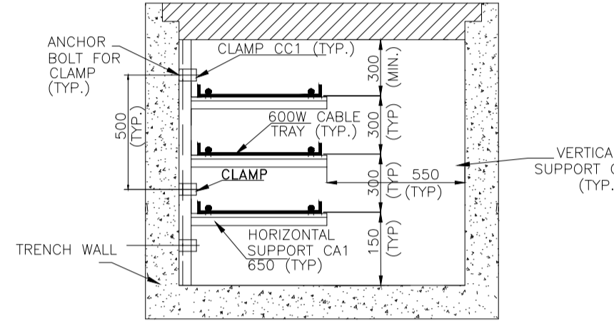
TRENCH DETAIL 1200WX1050D TR D-D
