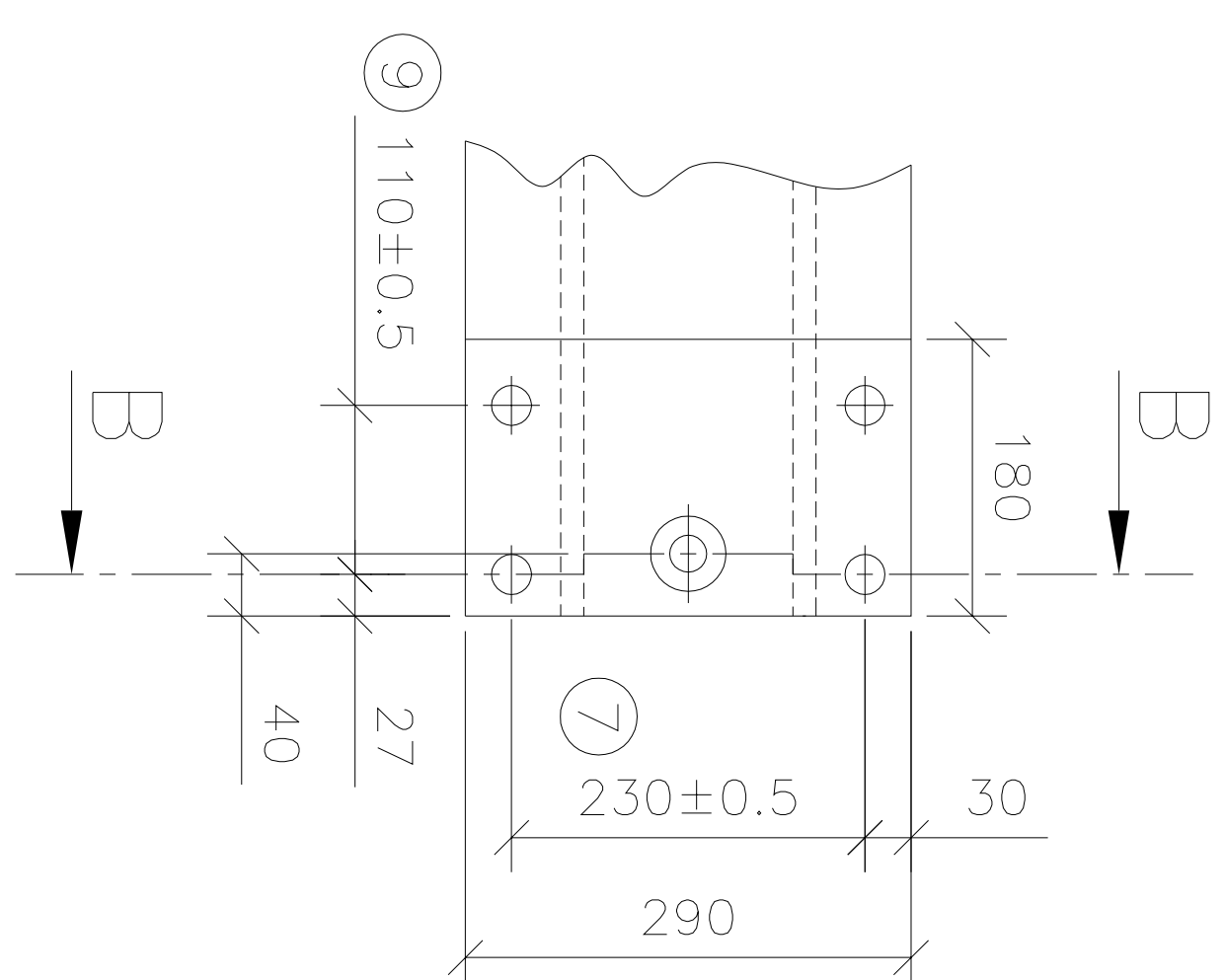
VIEW - X
