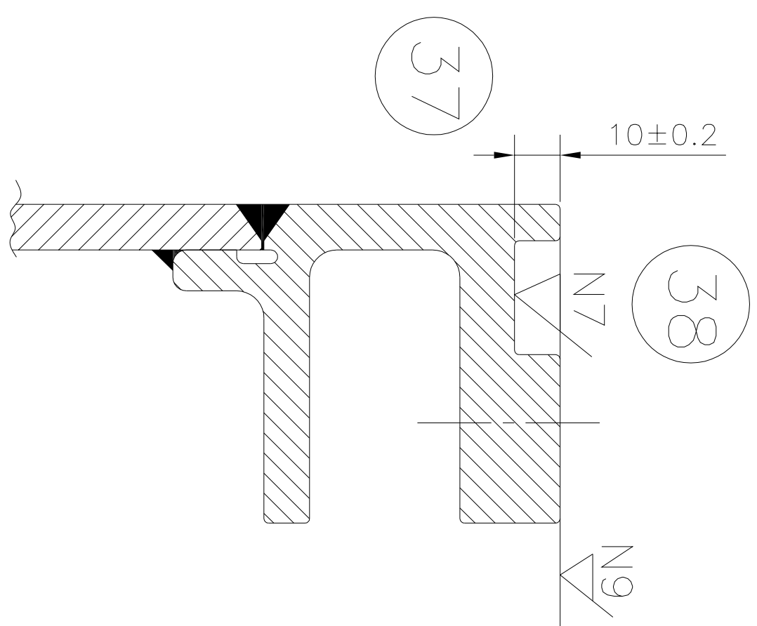
SECTION - CC
