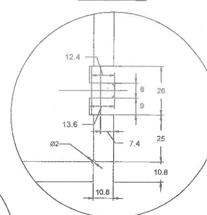
DETAIL "C"
