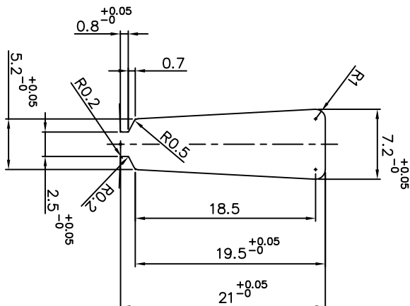
DETAIL-'X'
