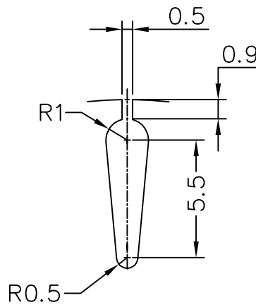
DETAIL-'A'
