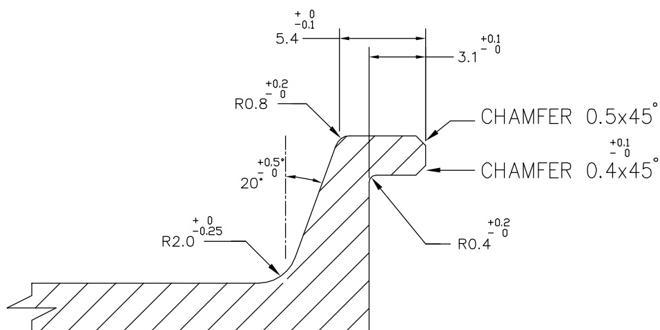
DETAIL - BB
