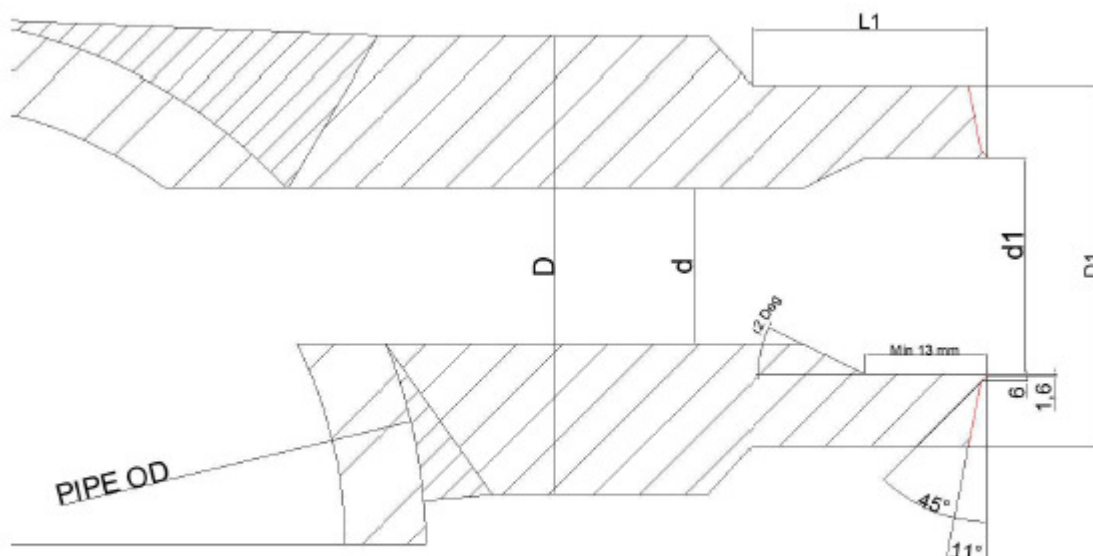
SKETCH 2 – MACHINING SKETCH DIMENSIONS AS PER TABLE 1 – RED COLOR HIGHLIGHTED AFTER FACING 20 mm
