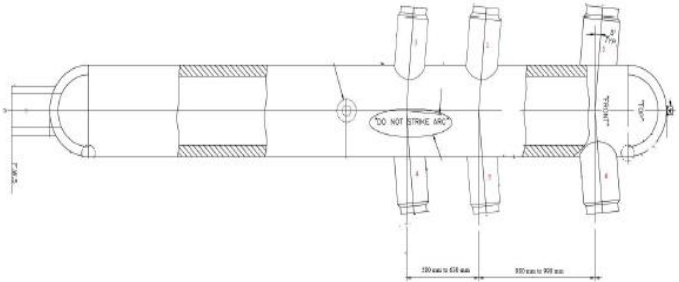
GENERAL ARRANGMENT OF VESSEL WITH WELDED NOZZLES NOZZLE 1 to 7 (as indicated) ARE TO BE MACHINED
