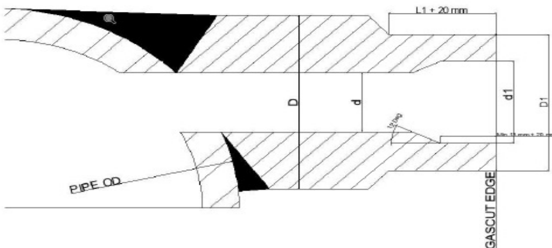
SKETCH 1 – AS GASCUT EDGE NOZZLE AFTER HYDRO TEST BEFORE MACHINING
