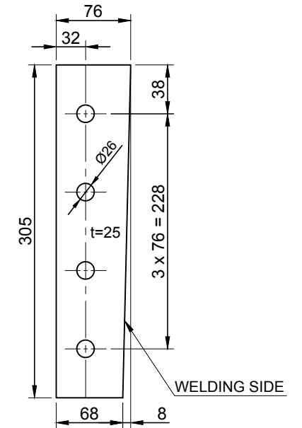
SUPPORT BAR
