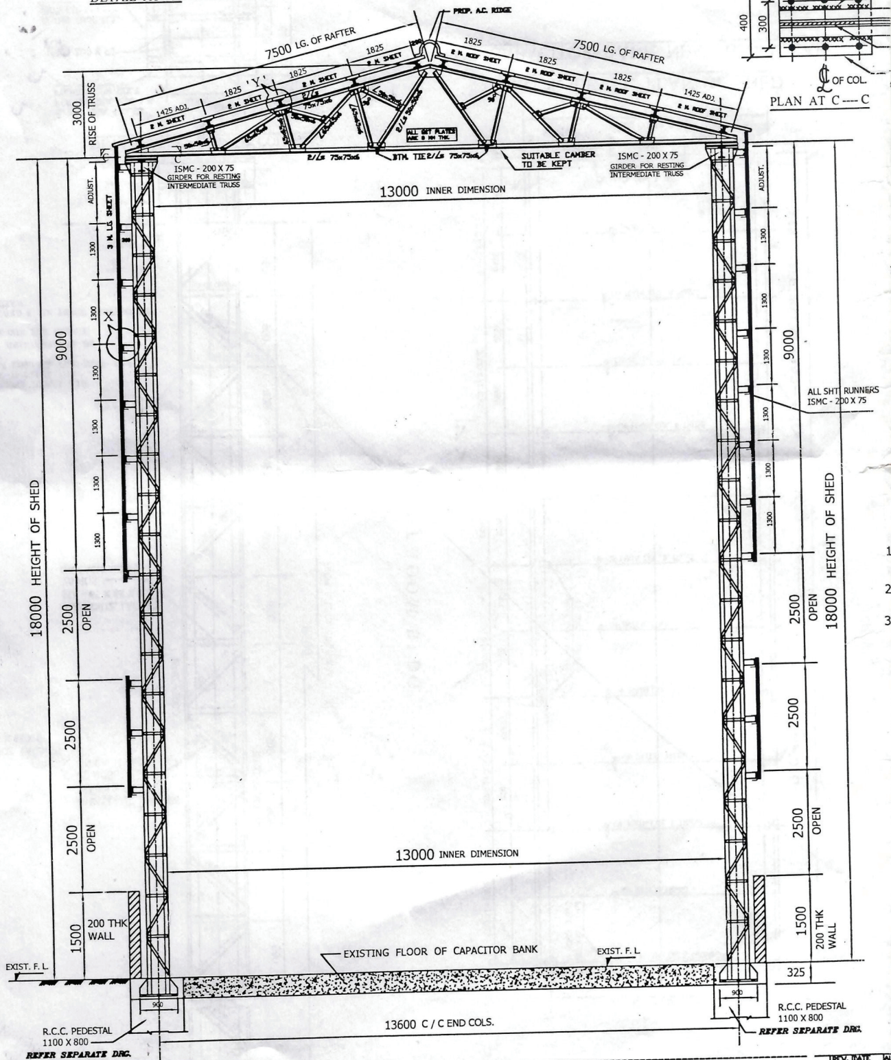
ENLARG. SECTION AT A --- A
