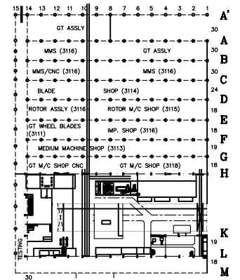
KEY PLAN OF 01 SHOP
